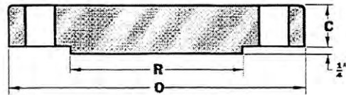
BLIND
