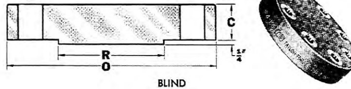
BLIND
