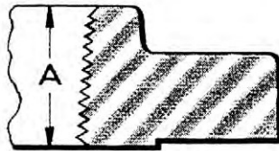
150 LB. STANDARD WITH 1/16" RAISED FACE
