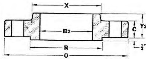
SLIP-ON
