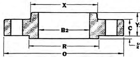
SLIP-ON
