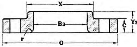
LAP JOINT
