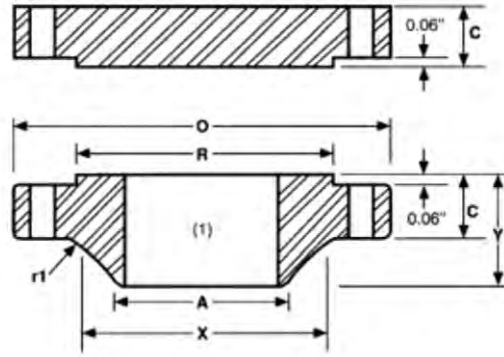
Class 900
