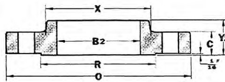
SLIP-ON
