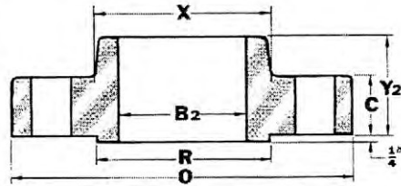
SLIP-ON
