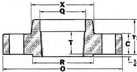
THREADED
