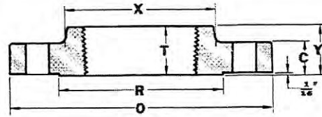
THREADED
