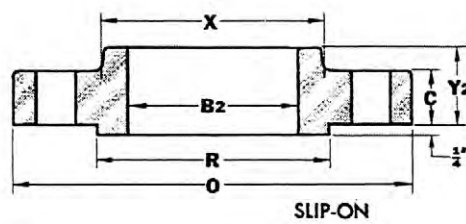
SLIP-ON
