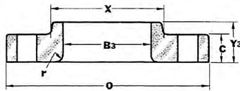
LAP JOINT
