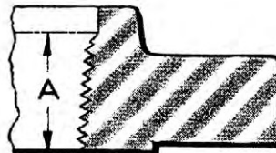
300 LB. STANDARD WITH 1/16" RAISED FACE
