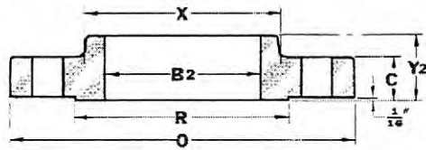
SLIP-ON
