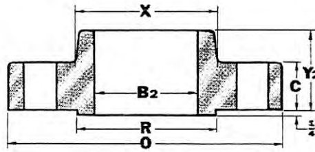
SLIP-ON
