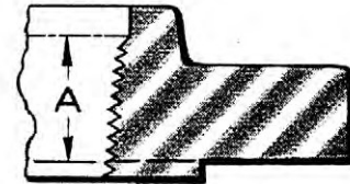
400 LB. STANDARD AND HEAVIER WITH 1/4" RAISED OR MALE FACE
