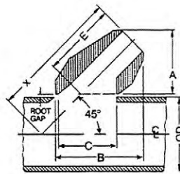
BUTT WELD
